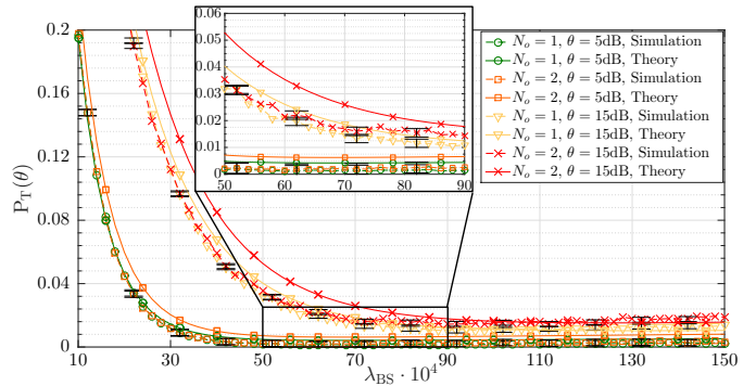
Fig. 5. SINR outage probability P_{\text{T}} as a function of the BS density \lambda_{\text{BS}} , for \theta \in \{5 \text{ dB}, 15 \text{ dB}\} dB, N_o = \{1, 2\} , \alpha_{\text{N}} = 4 , \psi = 30^\circ and G_{\text{TX}} = 20 \text{ dB} .
